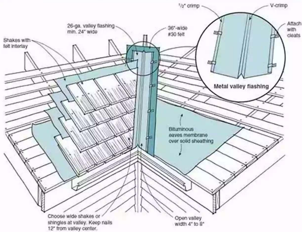
FIGURE 2-52 Valley Flashing for Shakes and Shingles.
